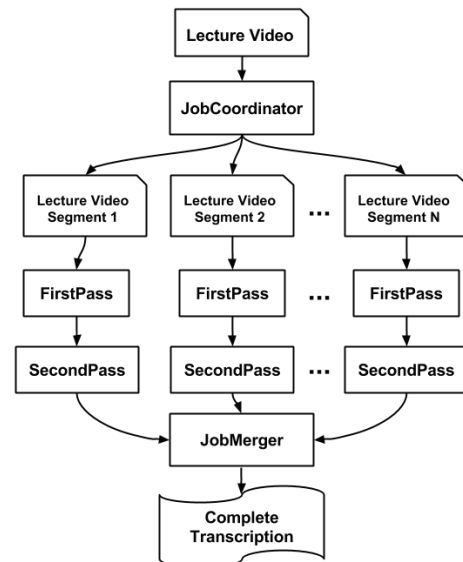
Figure 1: The ClassTranscribe transcription process.
