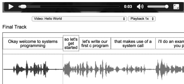
Figure 3: SecondPass transcription interface.
